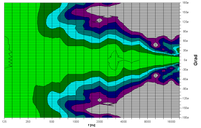
A1 vertikal - 2D Directivity Plot
