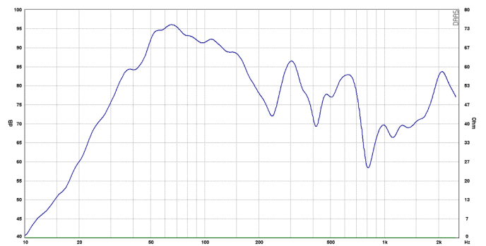
A1 Sub Frequenzgangkurve
