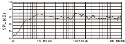
TREBLE Position (Straight ahead from the tweeter)
