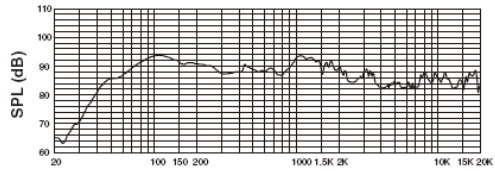
FLAT Position (Straight ahead from the tweeter)
