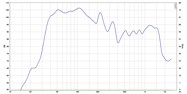
TSE infra Frequenzgangkurve
