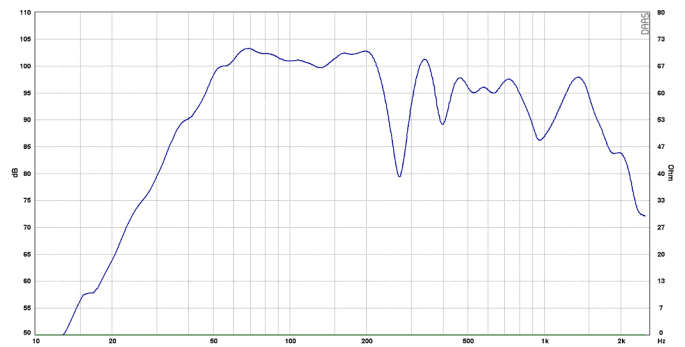
TSE Sub Frequenzgangkurve
