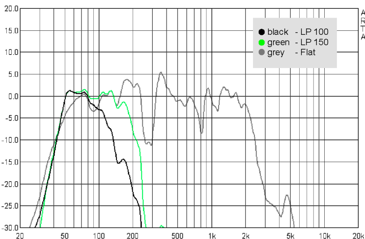
TSE Sub dp - Presets - Frequency response
