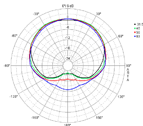
TSE Sub dp - Cardioid - polar diagram
