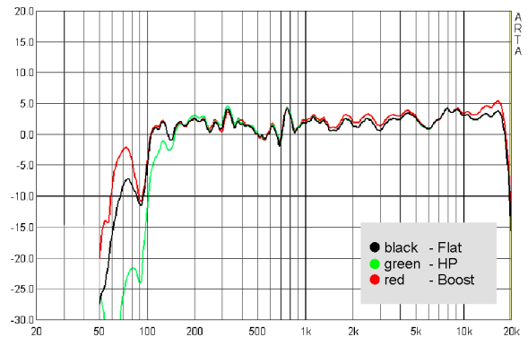
TSM10dp - Presets - Frequency response
