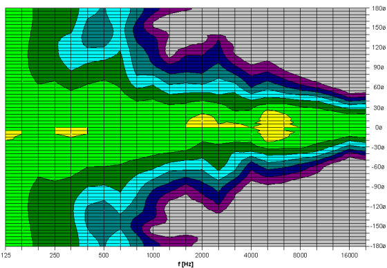
TSM10dp 90°x 60° horizontal - 2D Directivity Plot
