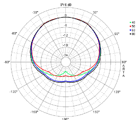
TSM Sub dp+ - Cardioid - polar diagram
