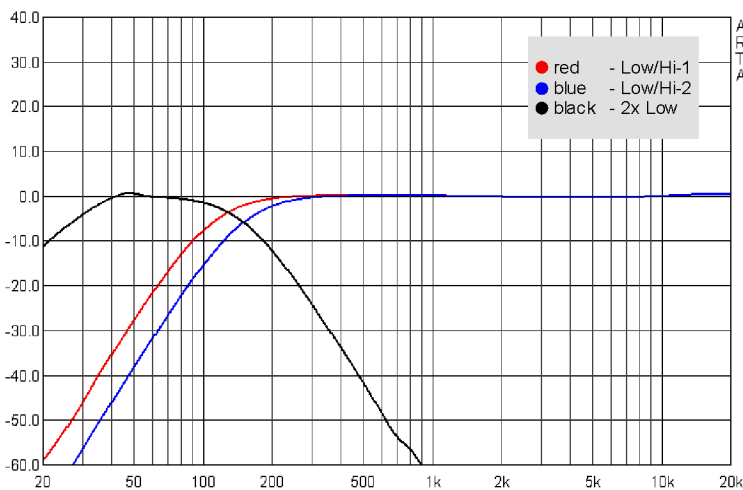
TSM Sub dp+ - Presets - Frequency response (electrical)
