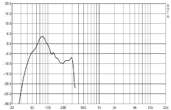
TSMini Sub dp - Frequency response
